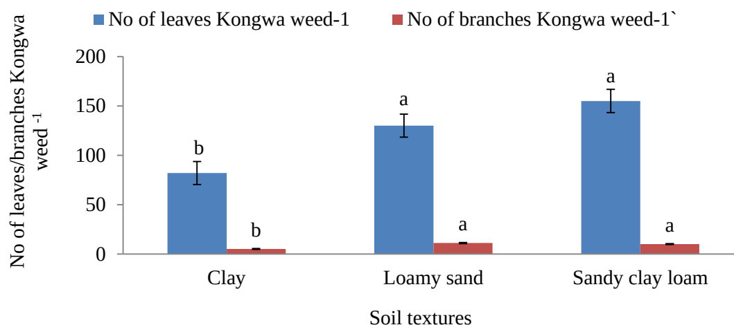
Figure 4: Effect of soil texture on leaves and branches of Kongwa weed among three soil textures
