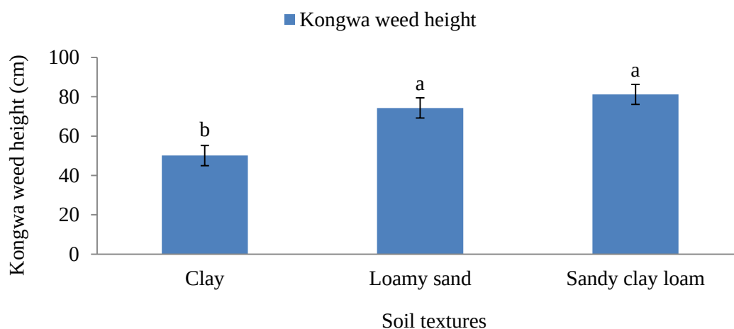
Figure 3: Effect of soil texture on Kongwa weed height among three soil textures
